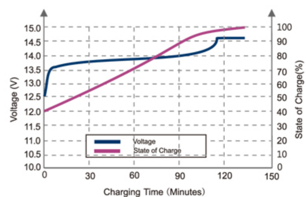
State of Charge Curve(0.5C, 25°C)
