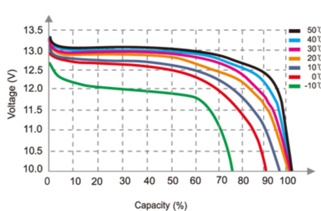
Different Temperature Discharge Curve(0.2C)
