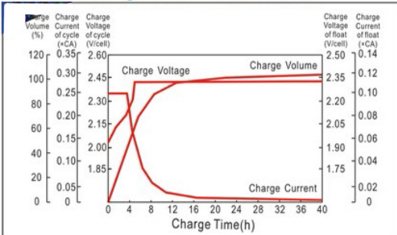
Charge Characteristics Curve
